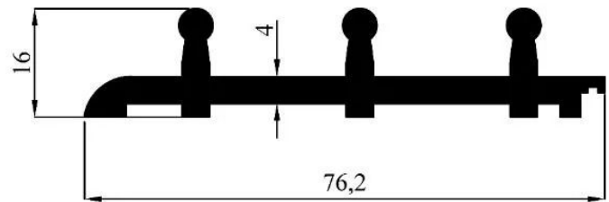
2392 1,212 kg/m
