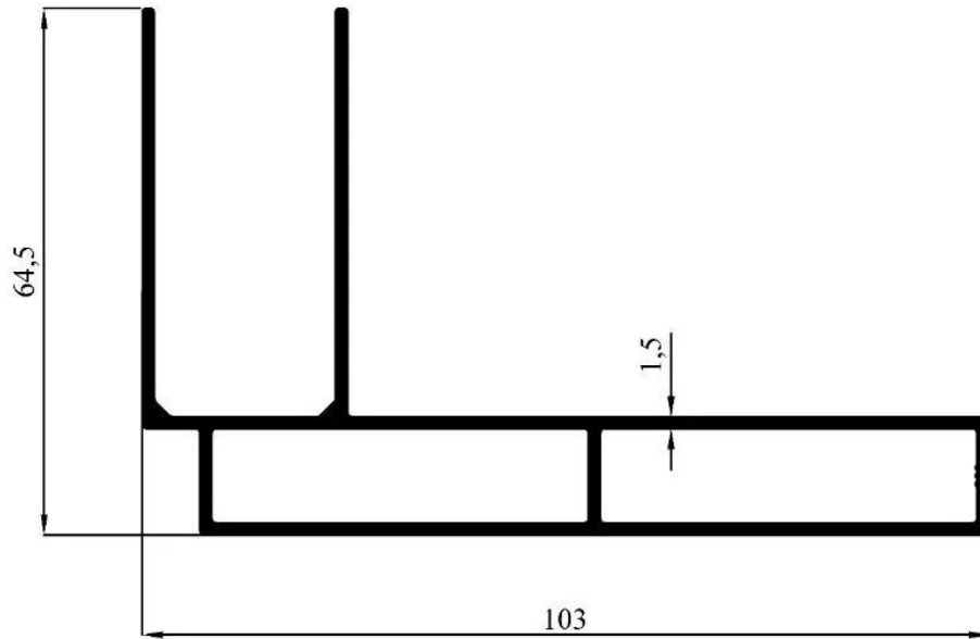
1792 1,367 kg/m
