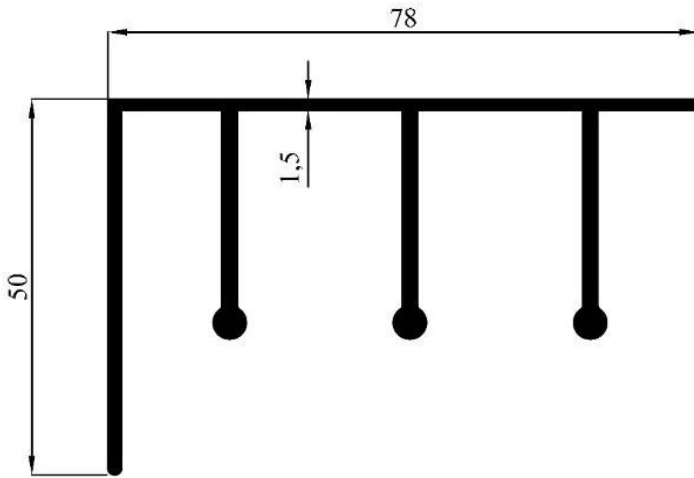
2389 1,103 kg/m
