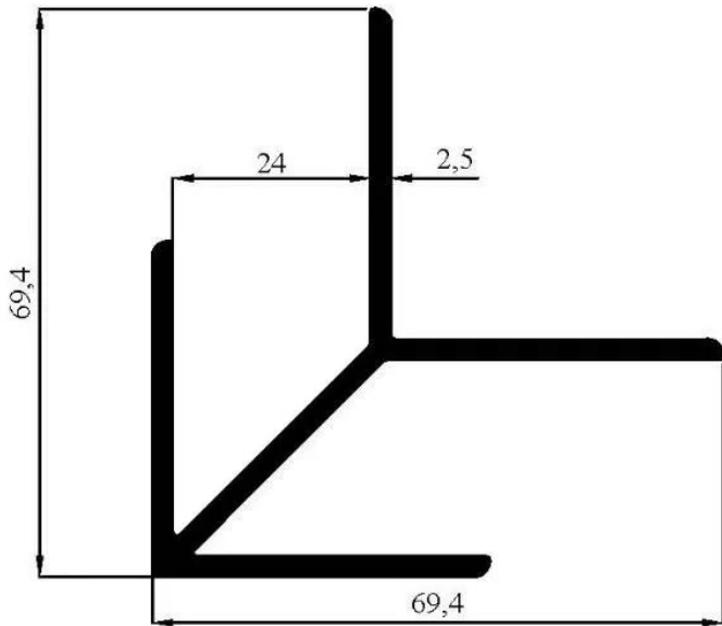
1589 1,325 kg/m
