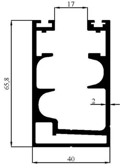
2338 1,577 kg/m
