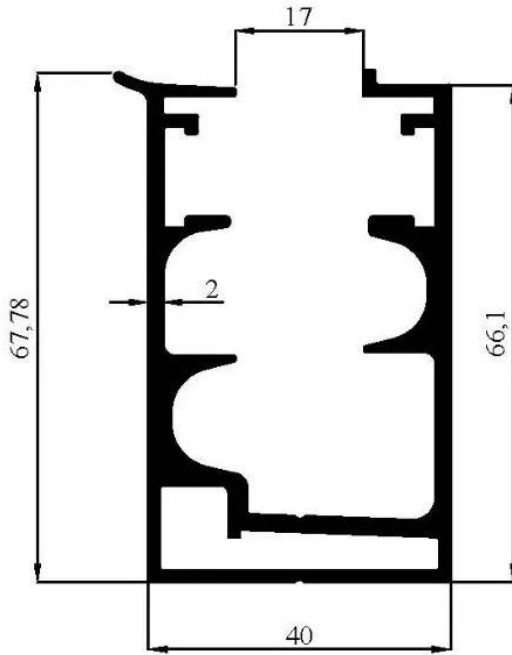
2337 1,569 kg/m
