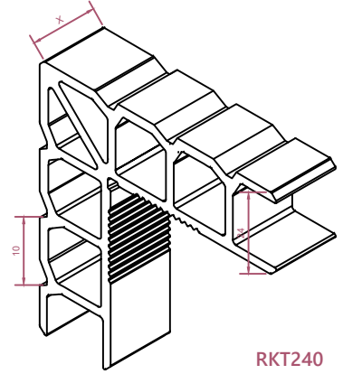
RKT240
