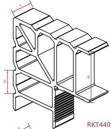
RKT440
